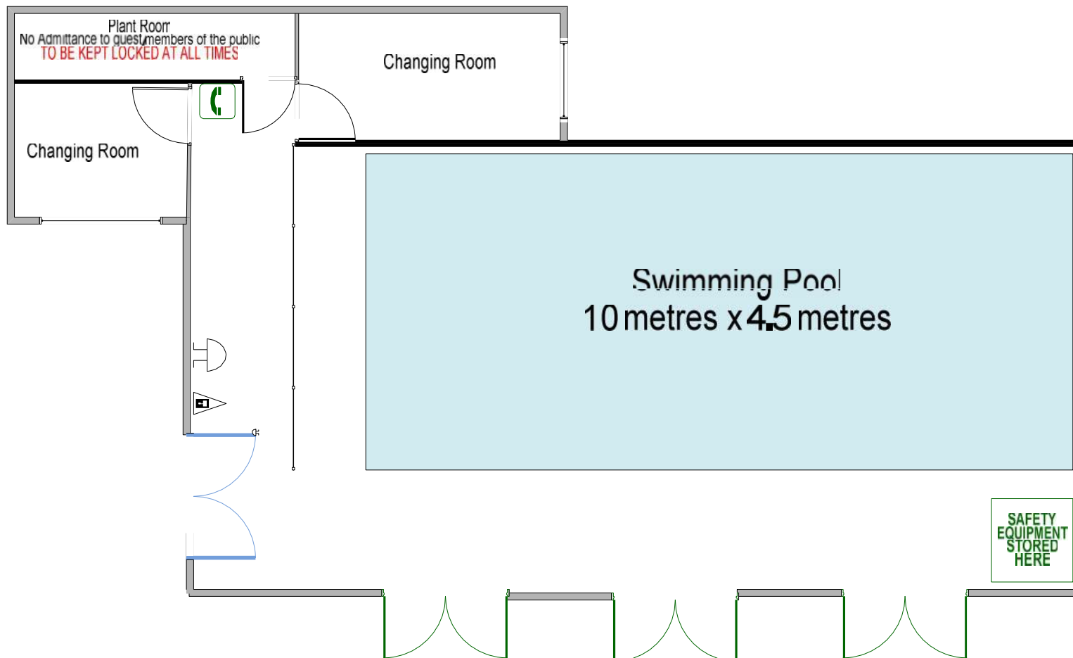
DIAGRAM OF THE POOL AND BUILDING ENTRY & EXIT DOOR [LIGHT BLUE] EMERGENCY EXIT DOORS [GREEN]
